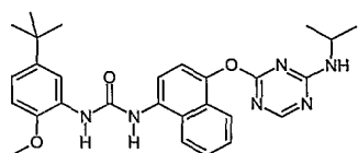
1-(5-tert-Butyl-2-methoxy-phenyl)-3-[4-(4-isopropylamino)-[1,3,5]triazin-2-yloxy]-naphthalen-1-yl]-urea;
